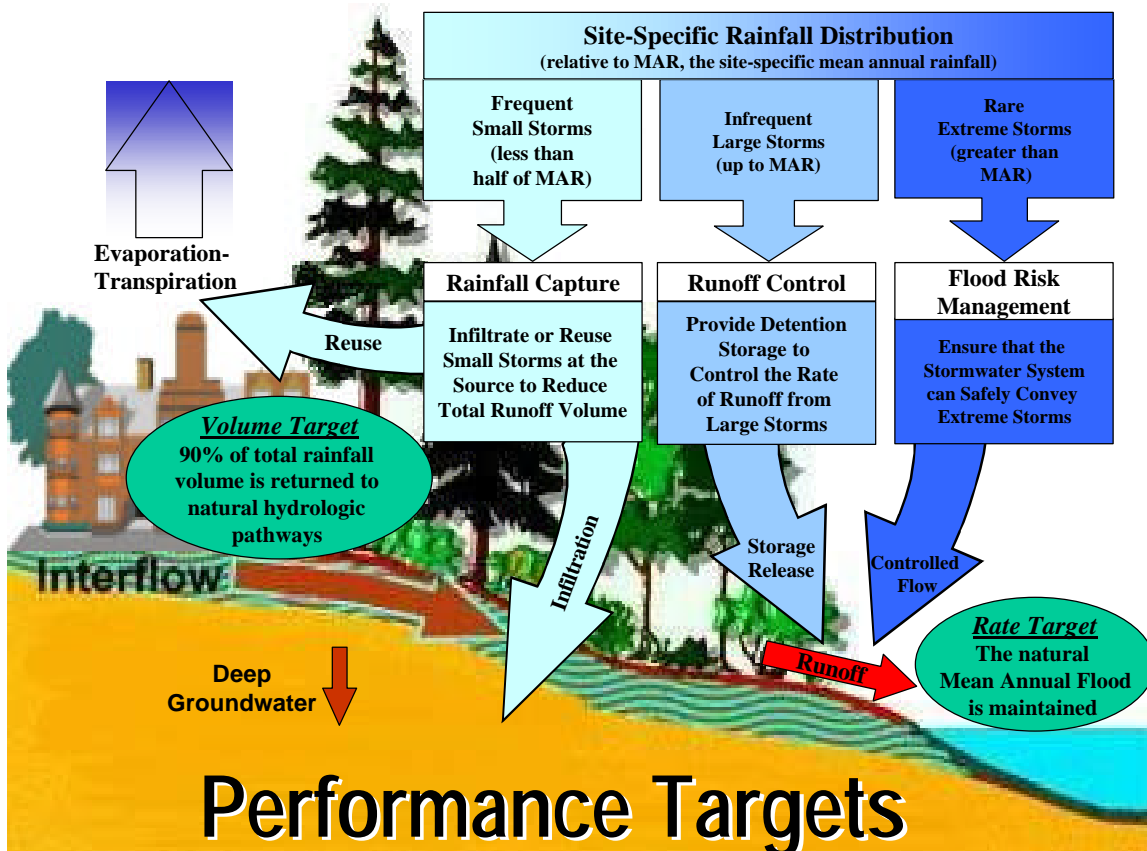
Figure 1. Managing the complete spectrum of rainfall events. Taken from Stormwater Planning: A Guidebook for BC (2002).
